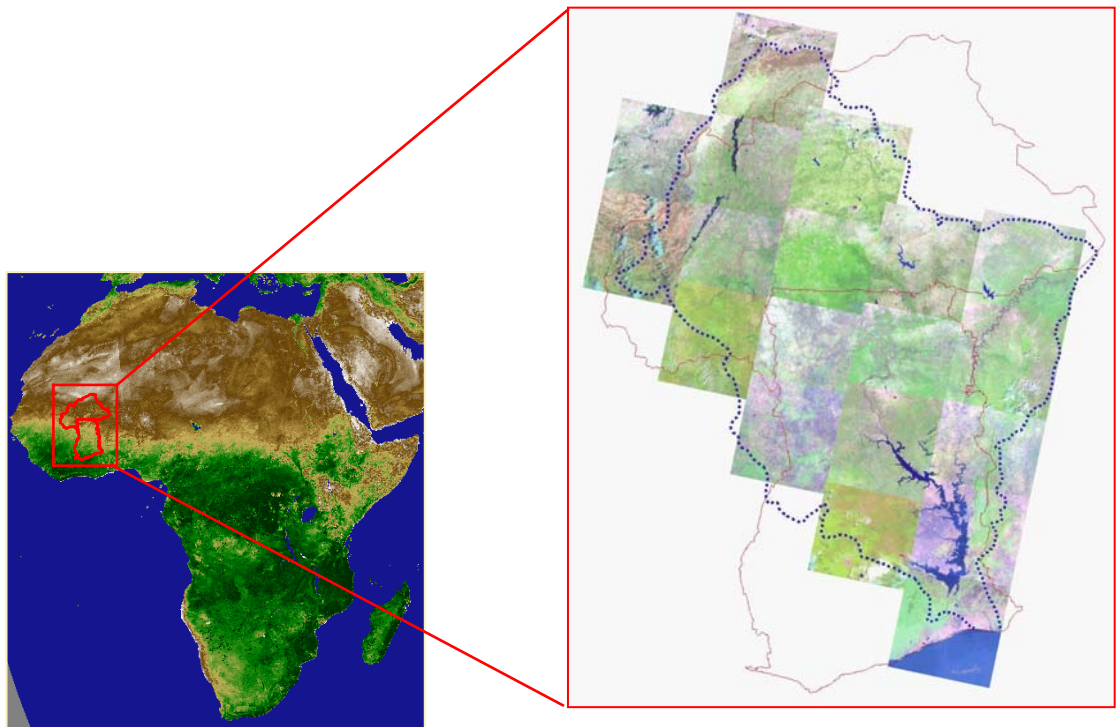
Figure 1 : NOAA-AVHRR satellite image composition ANSAT 1999-2000 images composition
