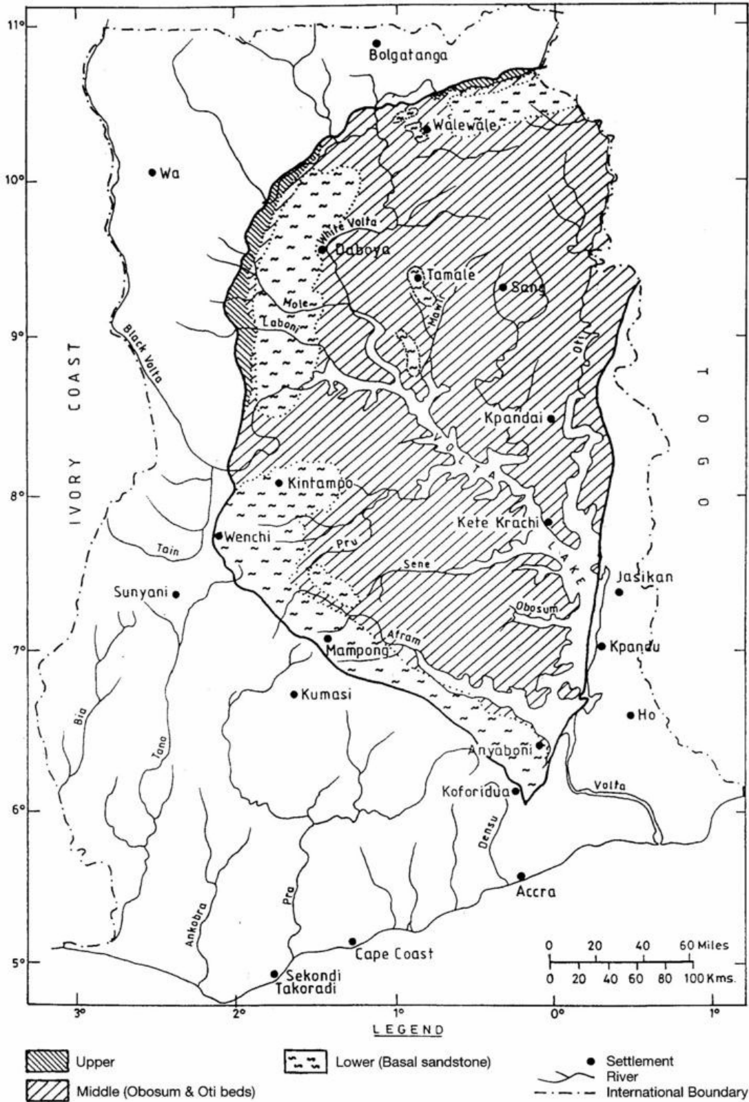
Figure 18: Hydrogeological subprovinces of the Voltaian System (Ghana Geological Survey 1965)
