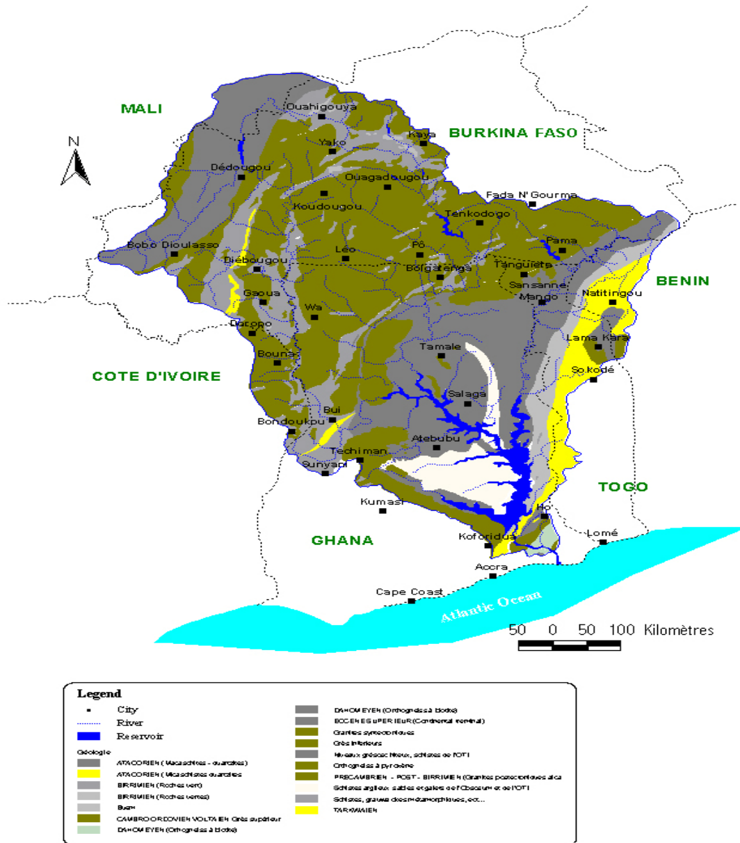
Figure 11: Geological Map of the Volta River Basin.
