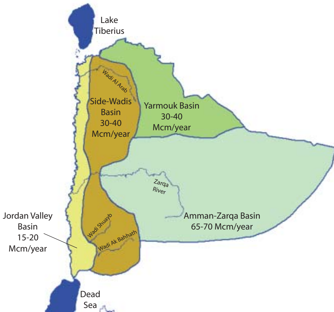
FIGURE 6. Groundwater basins in the LJRB in Jordan.
