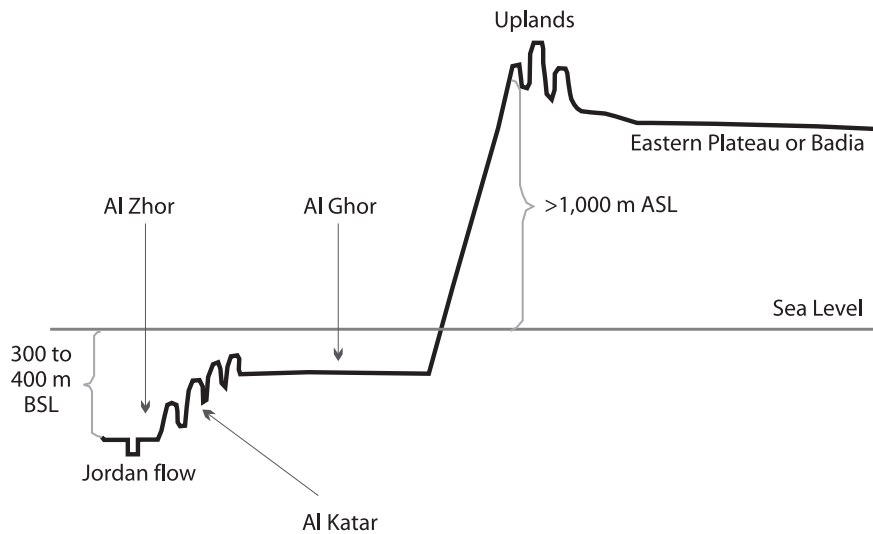
FIGURE 3. Topography of the LJRB in Jordan.
