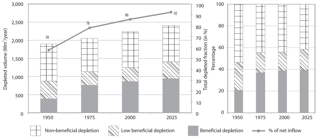
FIGURE 18. Evolution of depleted fractions in the LJRB (nominal values and percentage).
