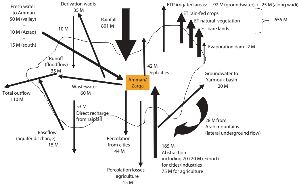
Balance of Zarqa Basin
