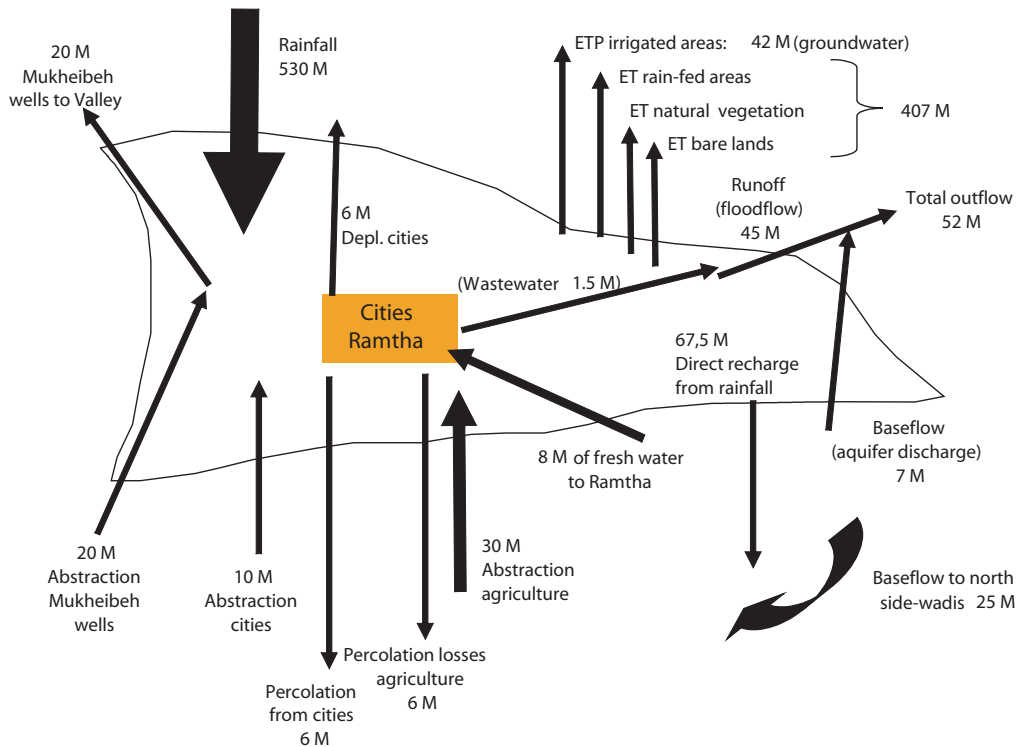
Balance of Yarmouk Basin
