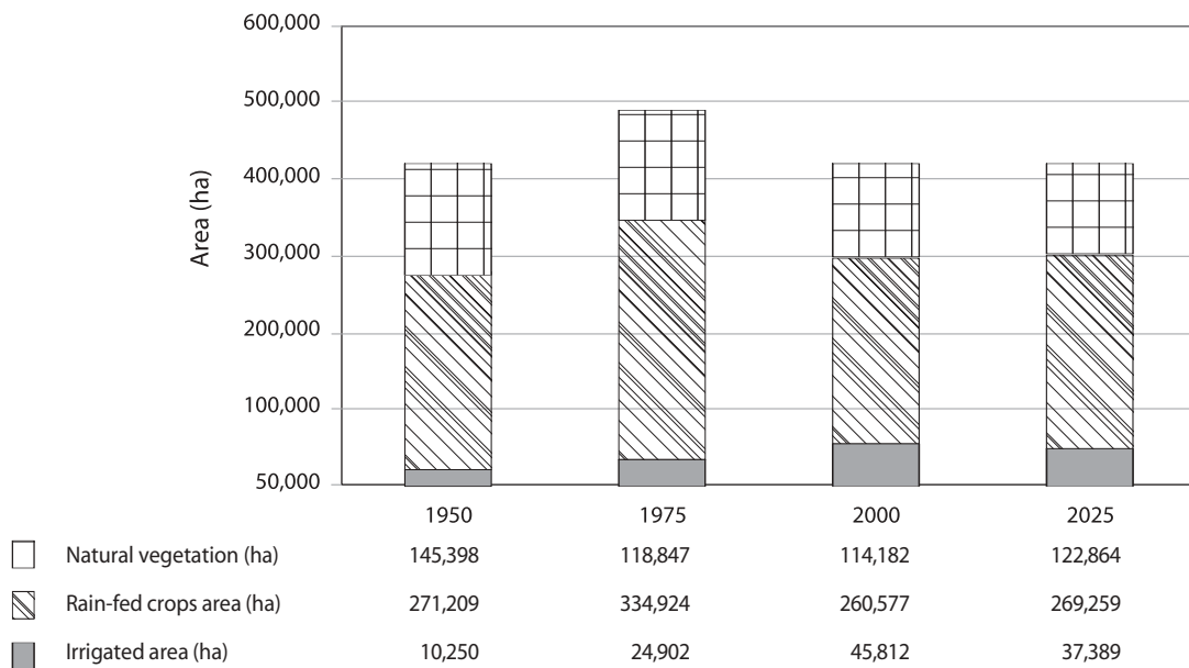
FIGURE 15. Evolution of vegetated areas in the LJRB in Jordan.
