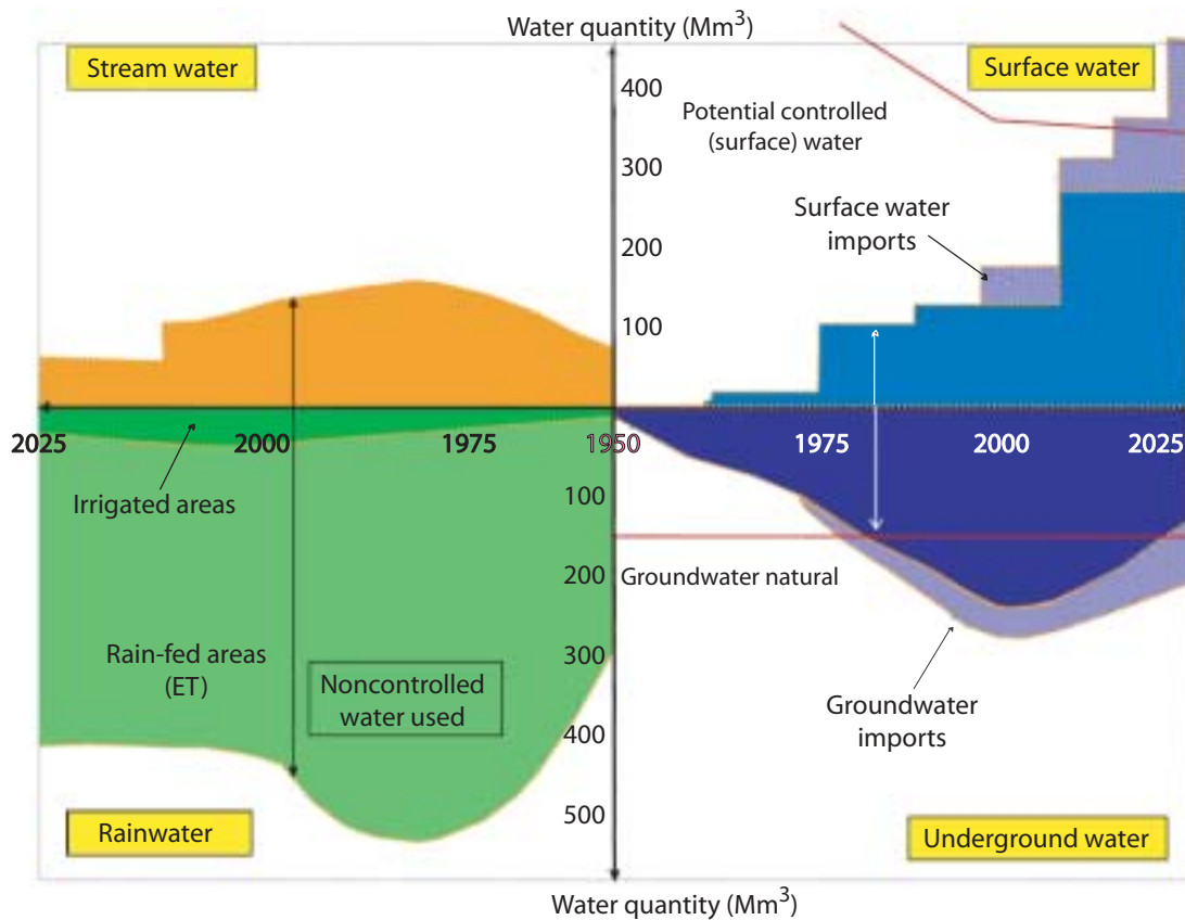
FIGURE 21. Four-quadrant diagram presenting water withdrawal trends in the LJRБ from 1950 to 2025 according to several water “categories.”
